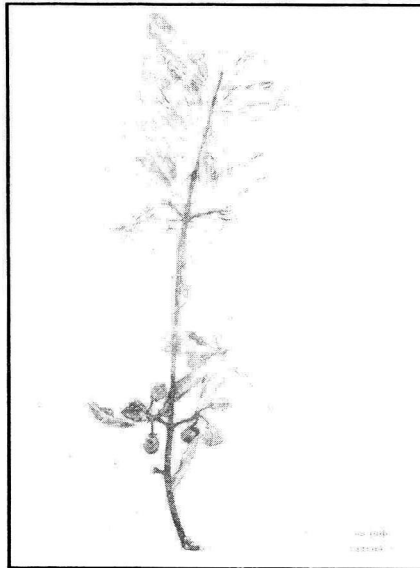
Symphonia globulifera
